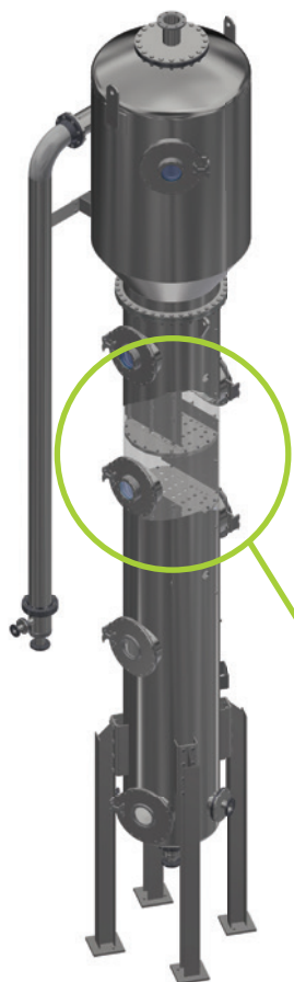
Crown Oil Stripper – Flex Control Trays
